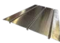
Emission Plate (1000x590x0.7mm)
