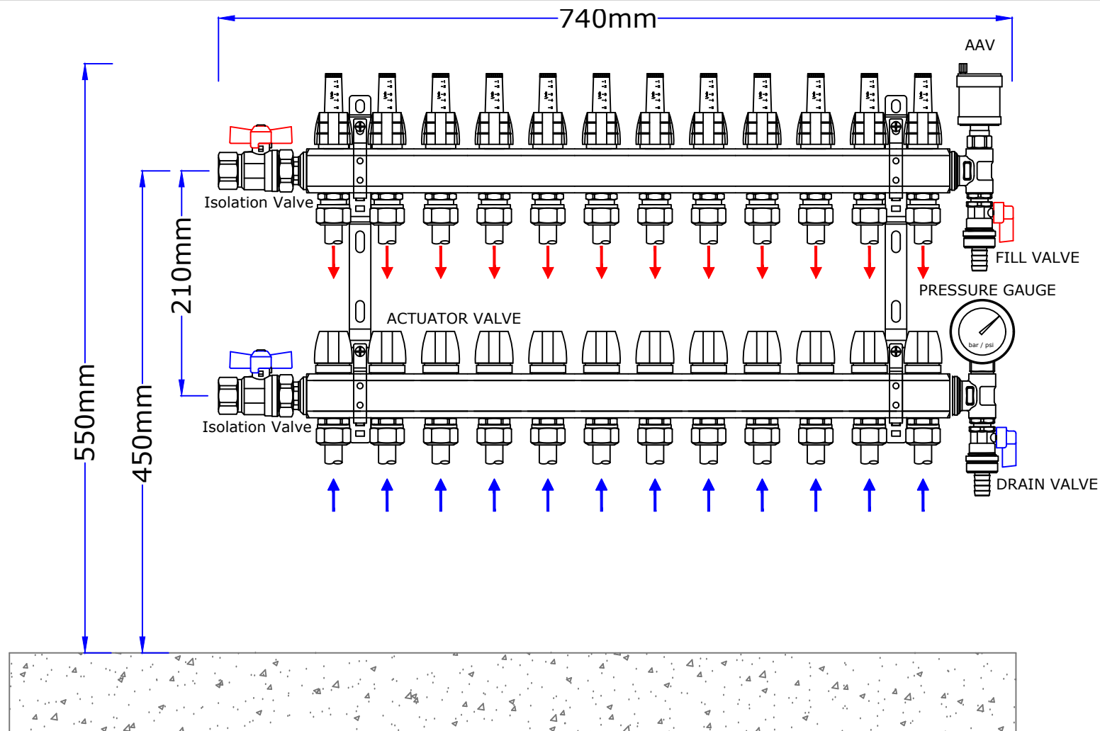
Luxusheat - Flow Meter Manifold
