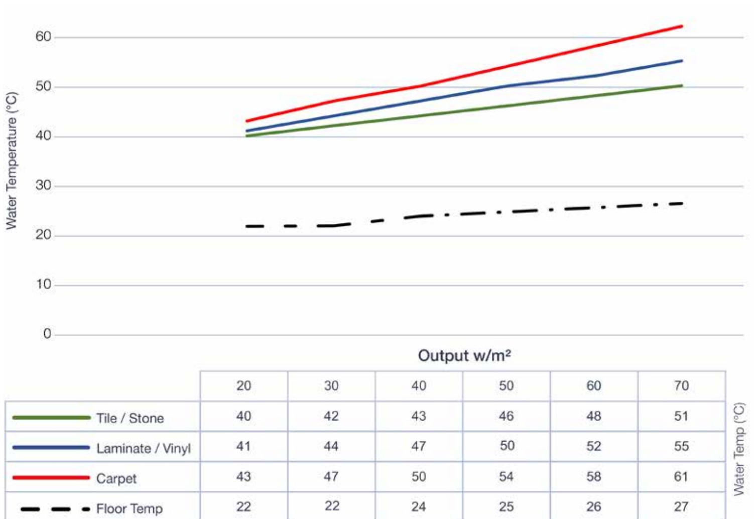
Heat output / Flow water Temperature (Slim 12 Light Tile)
